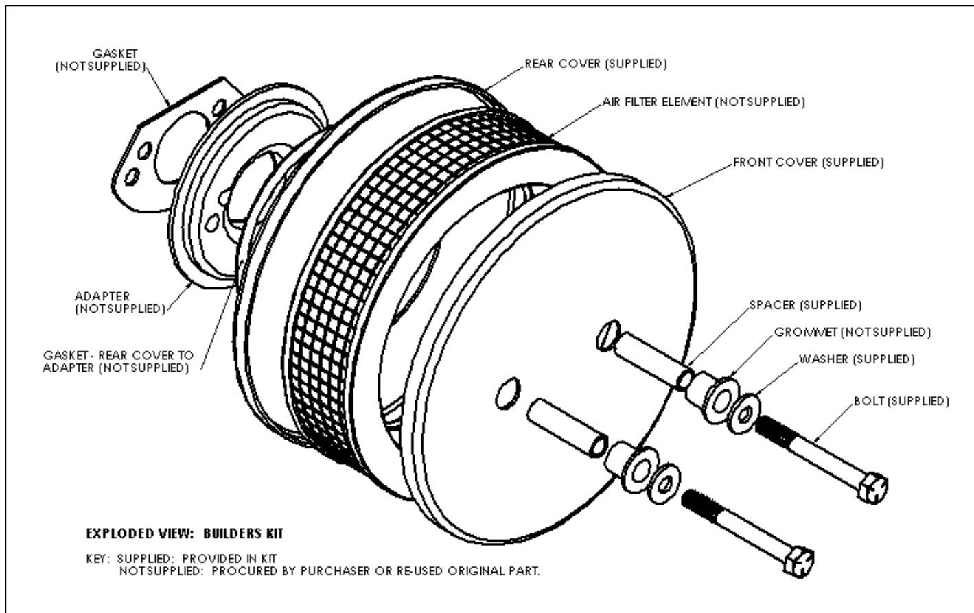
General arrangement of the builder's kit air cleaner assembly
